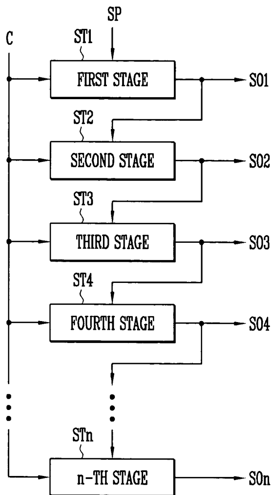
FIG. 1 (PRIOR ART)
