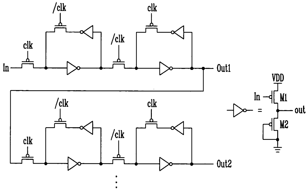
FIG. 2 (PRIOR ART)
